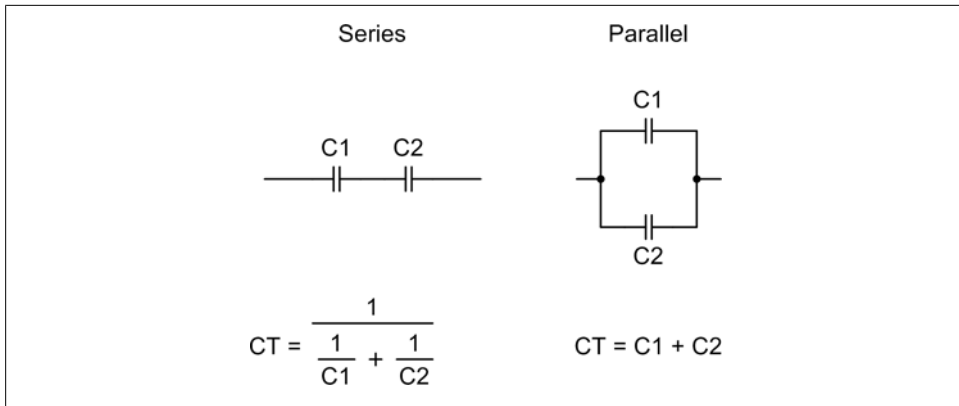
Figure 2-18. Series and parallel capacitance
