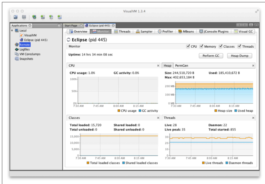
Figure 13-3. Monitor tab
