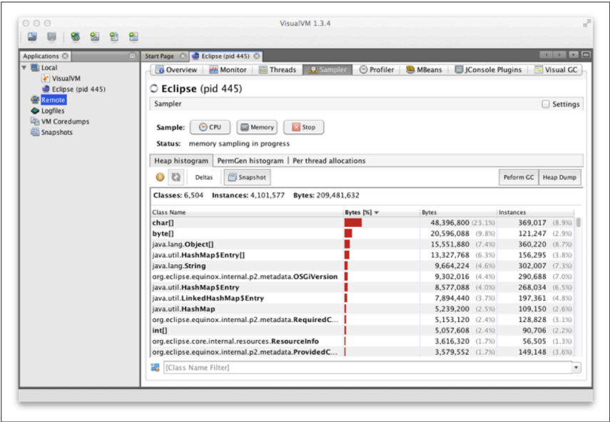
Figure 13-5. Sampler tab
