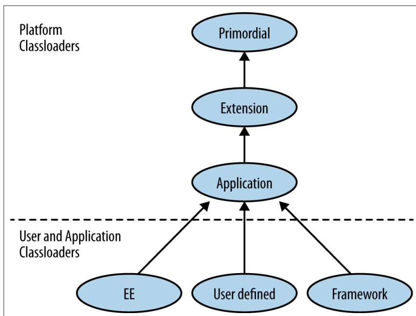
Figure 11-2. Classloader hierarchy
