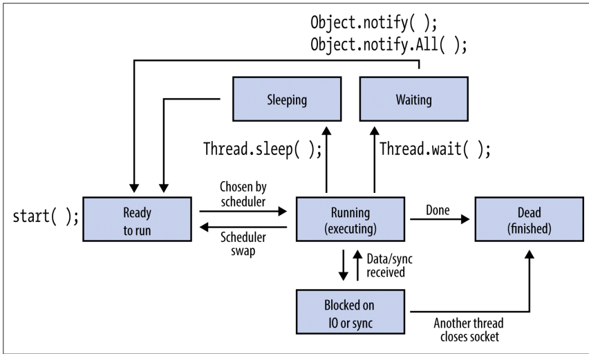
Figure 6-4. Thread lifecycle
