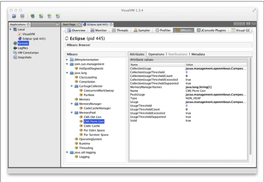
Figure 13-6. MBeans plug-in
