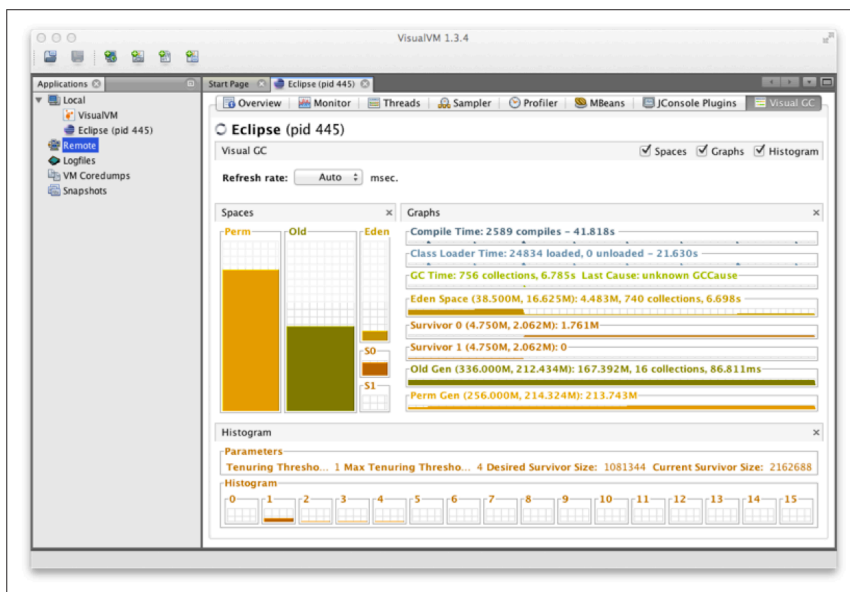
Figure 13-7. VisualGC plug-in
