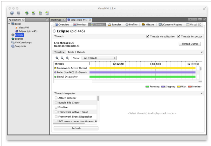
Figure 13-4. Threads tab
